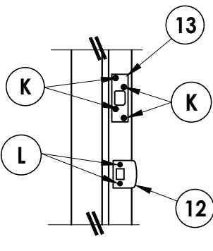
LATCH & DEADBOLT STRIKE PLATE DETAILS
