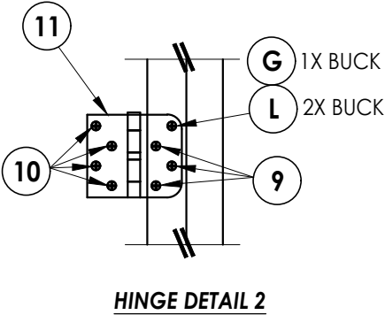
HINGE DETAIL 2
