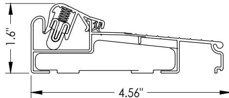
T8 INSWING ARTICULATING THRESHOLD ZACLAA4565
