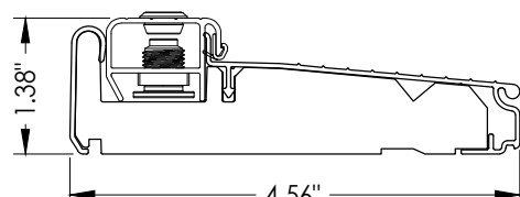
T4 INSWING ADJUSTABLE THRESHOLD ZAI4565FN
