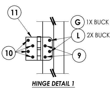
HINGE DETAIL 1
