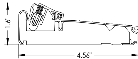
T9 INSWING ARTICULATING THRESHOLD ZACAA4565FN
